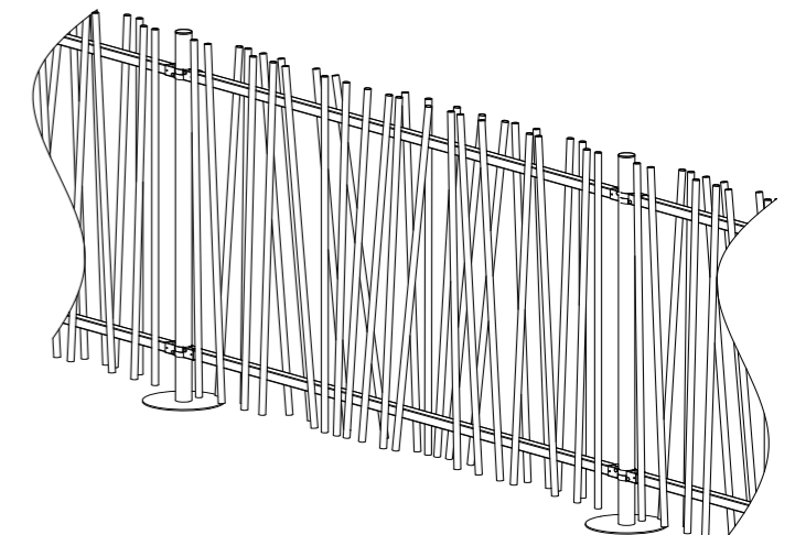
Step 6 Repeat as many times as necessary. If base plate anchoring has been used instead of foundation anchoring, screw on the base and insert the first post. Hook in the panel and insert the next post.
