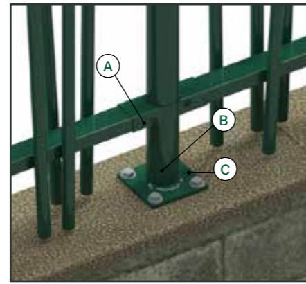
BASE PLATE A base plate can be used to install the posts on the concrete wall, or for fences less than 2m high. A. Nature fence post B. Base plate C. Anchor
