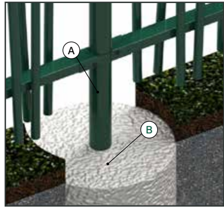
FOUNDATION Post installation with concrete footings A. Post Nature B. Foundation
